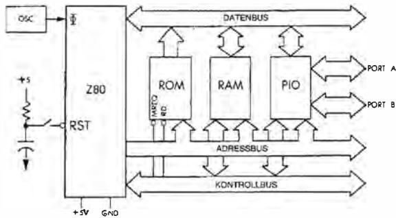
Abb. 2.1: Z80-Standardsystem
